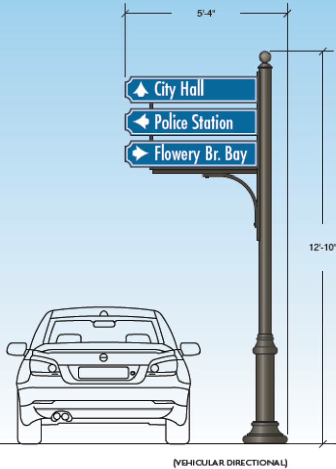
Vehicular Directional
